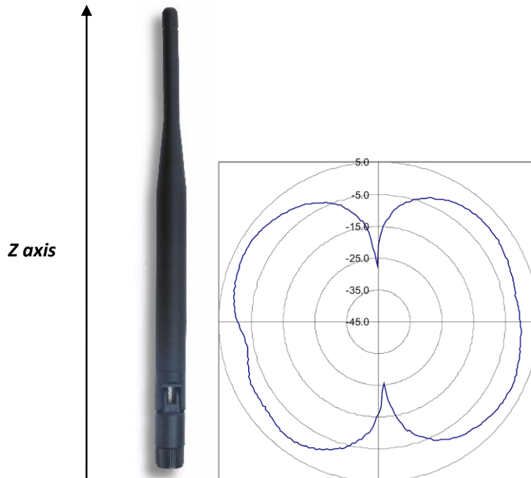
Figure 5: Half-Wave Dipole Antenna
