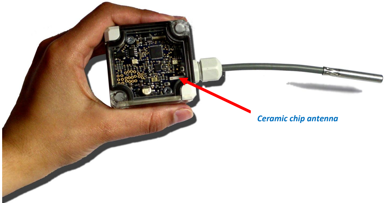
Figure 1: A BeanDevice SUN-T with an internal ceramic chip antenna
