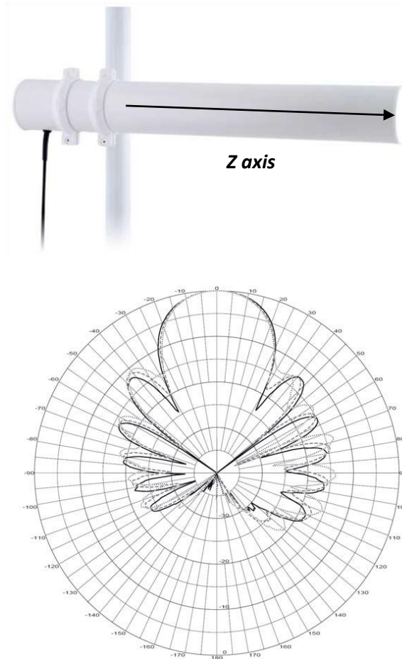
Figure 6: Yagi Antenna
