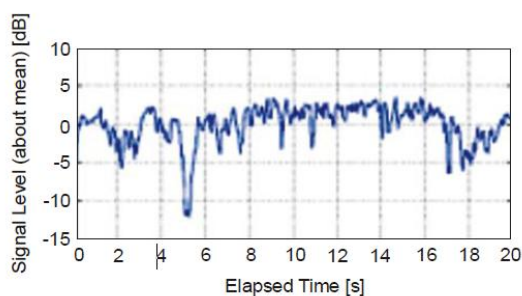
Figure 8: Multipath Fading Over Time
