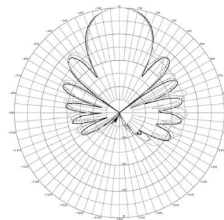
Directive Antenna
