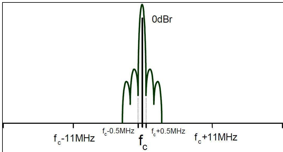
Figure: Bluetooth spectral Mask
